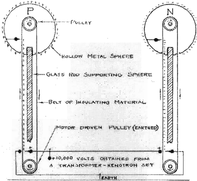
DIAGRAM OF FIRST GENERATOR
